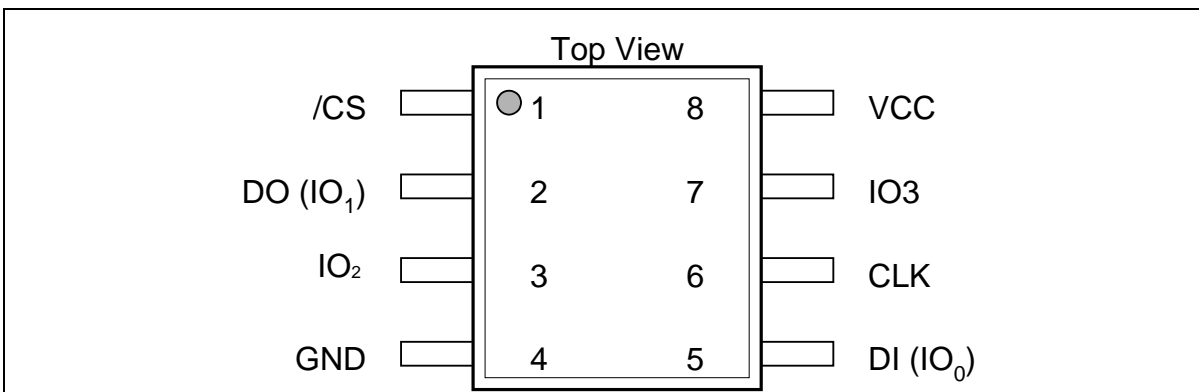
Figure 1a. W25Q32JV Pin Assignments, 8-pin SOIC 208-mil (Package Code SS/ ST)
