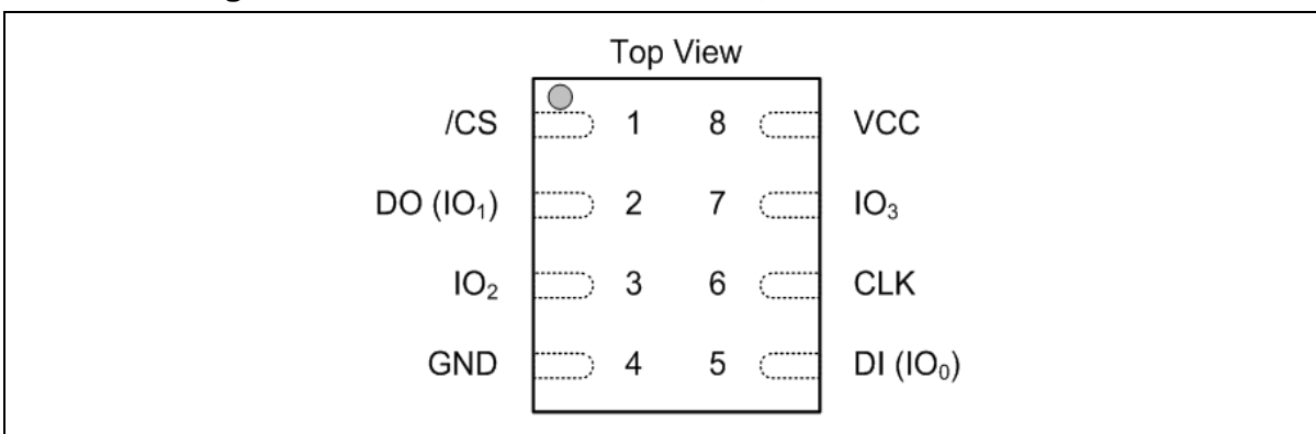
Figure 1b. W25Q32JV Pad Assignments, 8-pad WSON 6x5-mm (Package Code ZP/ZE, XG)
